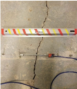
Crackmeter installation
